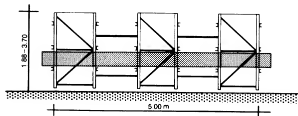
8 Continuous bracket racking
